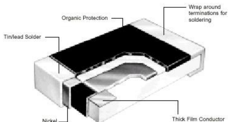
Fig1, Ceramic chip resistor construction
